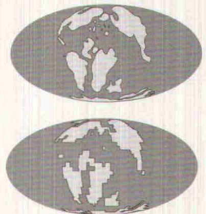
Figure 7: Degrading of coastal resolution (from top to bottom) as an indication of the uncertainty in model produced mid-cretaceous ocean flows.
